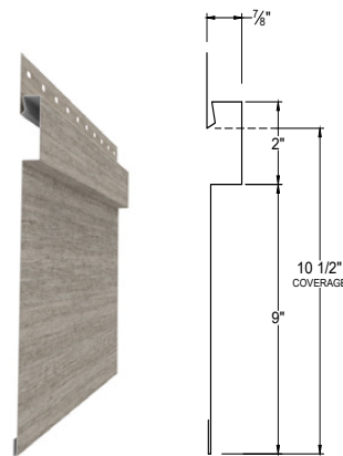
BOARD & BATTEN (497)
