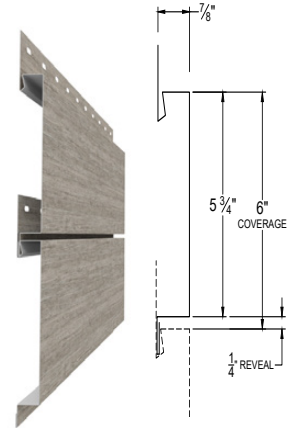
SHIPLAP (498)
