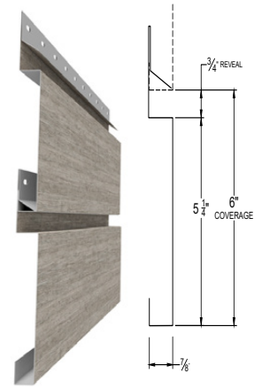
REVEAL (501)
